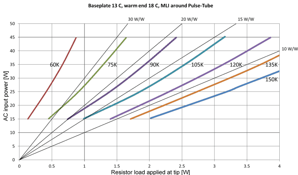
Figure 5. Heat lift at 13 C base plate temperature
