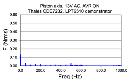
Figure 9. Exported vibrations (compressor axis), AVR ON
