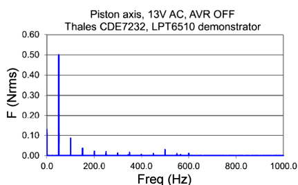
Figure 8. Exported vibrations (compressor axis), AVR OFF
