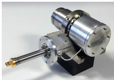
Figure 4. Demonstrator model.
