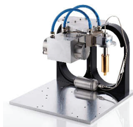
Figure 2. SSC80 pulse-tube for IPAG
