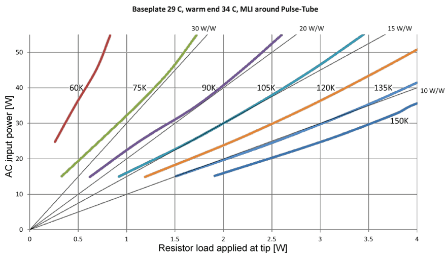
Figure 6. Heat lift at 29 C base plate temperature.
