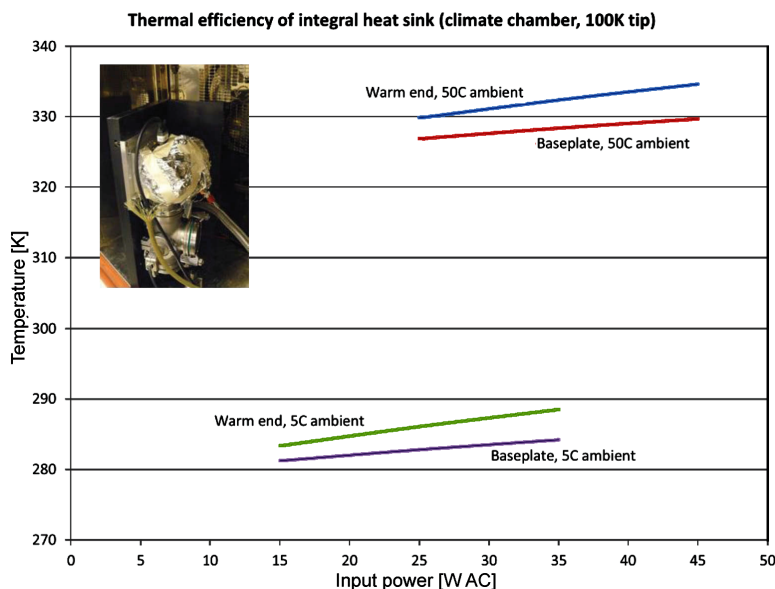
Figure 7. Efficiency of heat sinking through base plate
